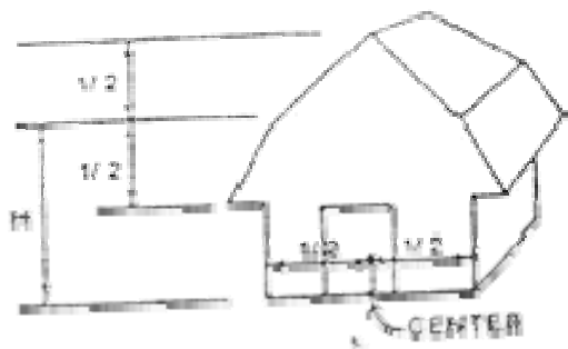
GAMBREL ROOF
