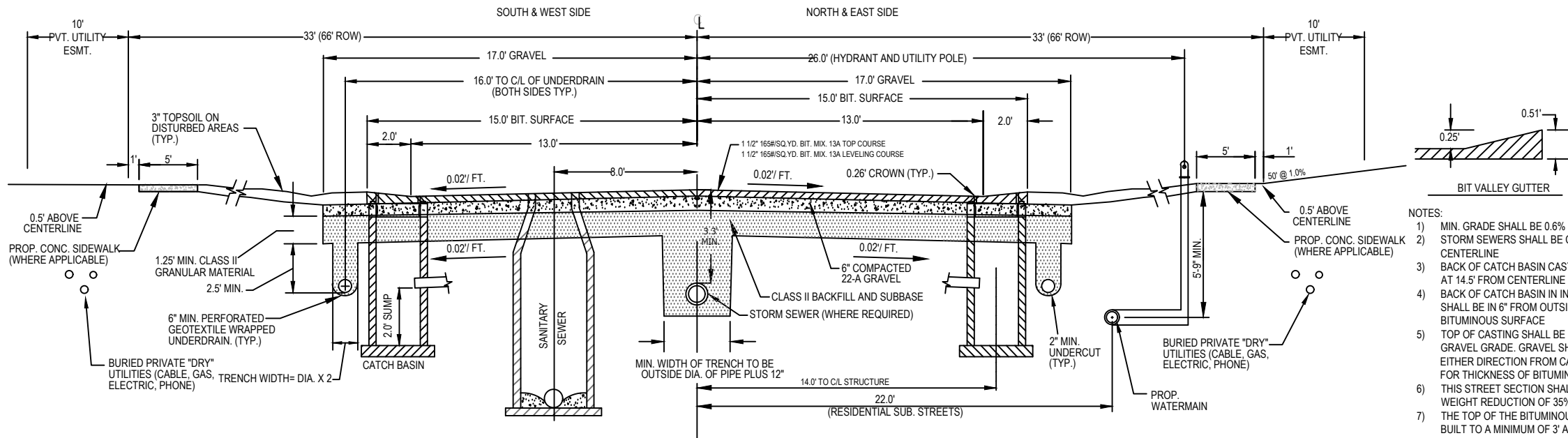
OTTAWA COUNTY ROAD COMMISSION TYPICAL RESIDENTIAL SECTION WITH BITUMINOUS CURB & INFRASTRUCTURE LOCATION PROFILE
